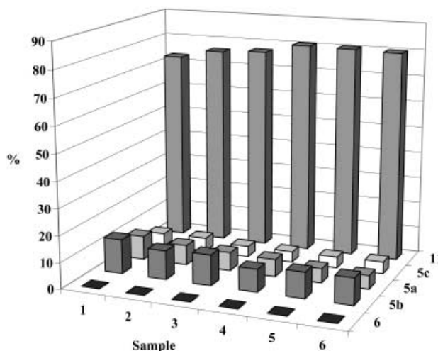
Figure 2. Plot showing the variation in selectivity of the aerobic oxidation reaction of 1,2,4-trimethylbenzene ( 10 ) in \text{scH}_2\text{O} observed during a continuous run. Samples were collected at 15 min intervals after the reactor had reached stable conditions. Catalyst strength: Mn 1719 ppm/Br 5000 ppm, flow rates: \text{H}_2\text{O}_2 (P-01): 8.19 mL/min, catalyst (P-02): 4.023 mL/min, organic (P-03): 0.061 mL/min, NaOH (P-04): 3.4 mL/min, temperature 380 °C and pressure 230 bar.
