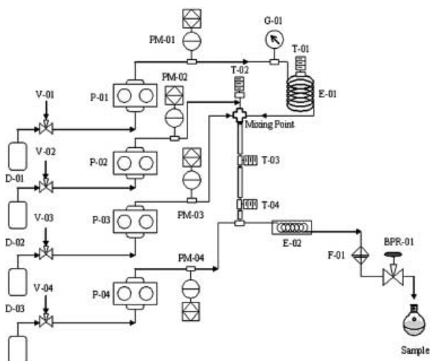
Figure 1. Configuration of the continuous aerobic oxidation reactor. D-01: water feed vessel, D-02: catalyst feed vessel, D-03: organic feed vessel, D-04: NaOH feed vessel, P-01: feed water pump (HPLC pump, Gilson model 305 Q-rate = 10 mL/min, \Delta P_{\max} = 60 MPa), P-02: feed catalyst pump (HPLC pump, Gilson model 305 Q-rate = 10 mL/min, \Delta P_{\max} = 343 bar), P-03: feed organic pump (HPLC pump, Gilson model 306 Q-rate = 5 mL/min, \Delta P_{\max} = 343 bar), P-04: feed NaOH pump (HPLC pump, Gilson model 303 Q-rate = 5 mL/min, \Delta P_{\max} = 343 bar), G-01: pressure gauge (Bourdon gauge), PM-01: pressure transducer and pressure monitor (water line), PM-02: manometric module, Gilson 802C, maximum pressure: 60 MPa (catalyst line), PM-03: pressure transducer and pressure monitor (organic line), PM-03: manometric module, Gilson 802C, maximum pressure: 60 MPa (NaOH line), T-01, T-02, T-03 and T-04: thermocouples, E-01: pre-heater (1/4 in AISI 316 tubing with 300 cm heat supplied by a cartridge heater (Watlow, 240 V, 200 W, FIREROD0247 NFRG2E164A) and a band heater (Watlow, 240 V, 200 W, NTB25X6UA3, 47 02 DM)), R-01: tubular reactor (1/4 in Hastelloy C276 pipe, 30 cm), E-02: cooler, F-01: 0.5 \mu m filter, BPR-01: Tescom, 26-1722-24-043 back pressure regulator max. P: 6000 psi.
