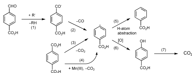
Scheme 3. Pathways leading to loss of methyl carbon atoms during autooxidation.
