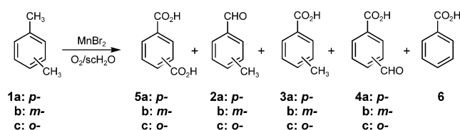
Scheme 1. Aerobic oxidation of xylene isomers in \text{scH}_2\text{O} .
