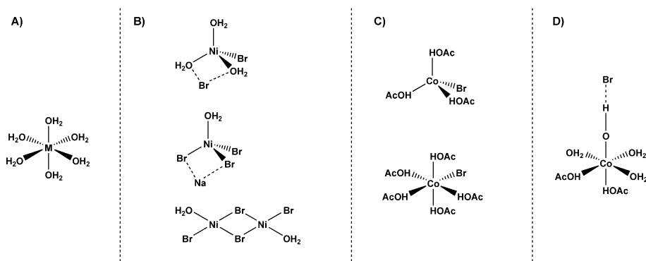
Figure 4. Predominant metal/bromide coordination compounds in active (scH 2 O, HOAc, H 2 O/HOAc) and inactive (non sc-water) solvents A ): in water M = Ni(II), Mn(II), Co(II). B ): In supercritical water. C ): In anhydrous acetic acid. D ): In hydrous acetic acid. Adapted from Refs. [31,35]
