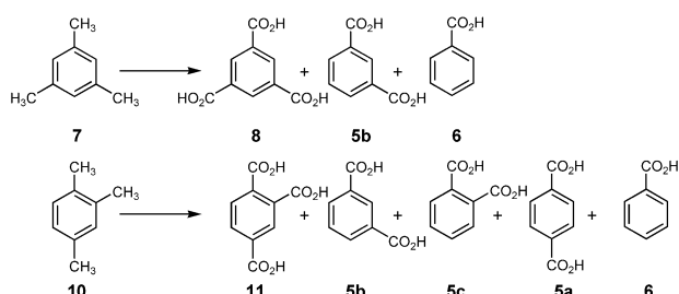
Scheme 2. Aerobic oxidation of trimethylbenzene in scH 2 O.
