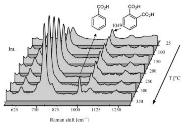
Figure 3. Raman spectra of an aqueous solution of 0.08 M phthalic acid and 0.04 M sodium hydroxide, heated isobarically at 300 bar stepwise from 25 to 350 °C. An NIR GaAlAs diode laser (785 nm) was used to excite the samples with \sim 300 \text{ mW} output power using an Almega (Thermo Nicolet) Raman spectrometer, exploiting 180° (back-scattered) geometry of scattering.
